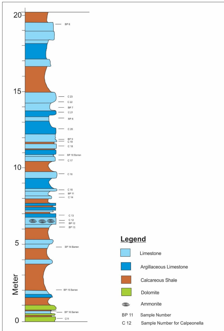
Figure-2: Stratigraphic column of the studied section, Banik Village, Dohuk Governorate, Kurdistan, and the location of studied samples (after Hakimi et al., 2015).
