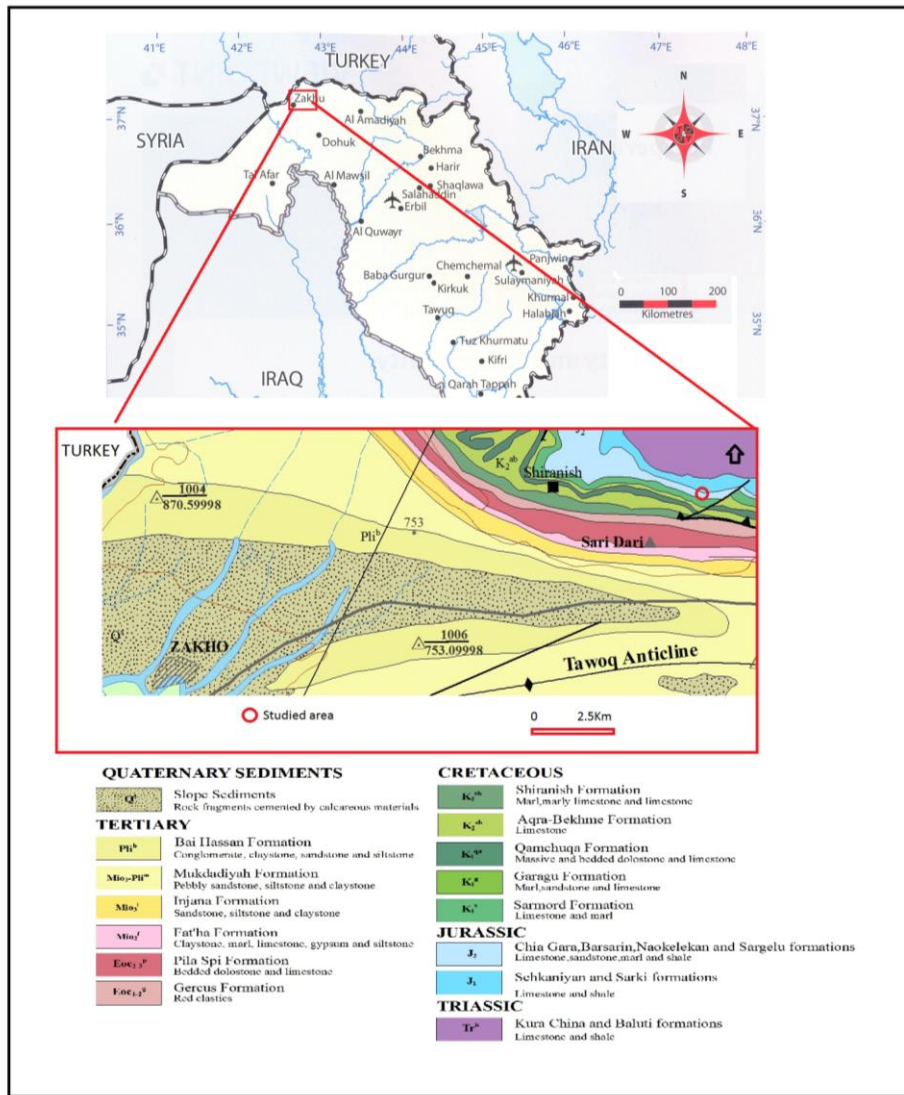
Figure-1: Location map for Banik Village in the Kurdistan Region, with a geological map of the studied area (modified after GEOSURV, 2012).
